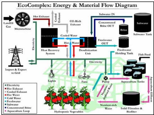
Figure 4 – New Jersey EcoComplex Installation & Schematic
