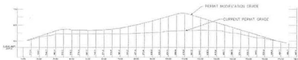
Figure 2. Section Profile Before and After Vertical Expansion
