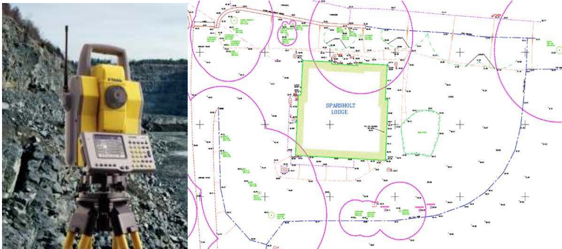
Figure 1. Total station
